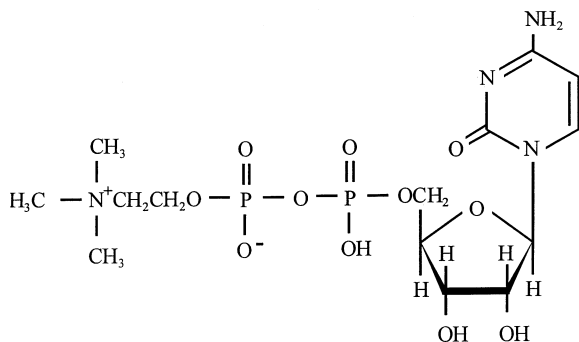
Fig. 1 Citicoline structure.
