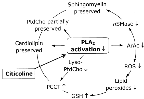
Fig. 3 Proposed major pathway of citicoline neuroprotection. ArAc, arachidonic acid; GSH, glutathione; nSMase, neutral sphingomyelinase; PLA 2 phospholipase A 2 ; PtdCho, phosphatidylcholine; ROS, reactive oxygen species. ↑ indicates increase; ↓ indicates decrease.
